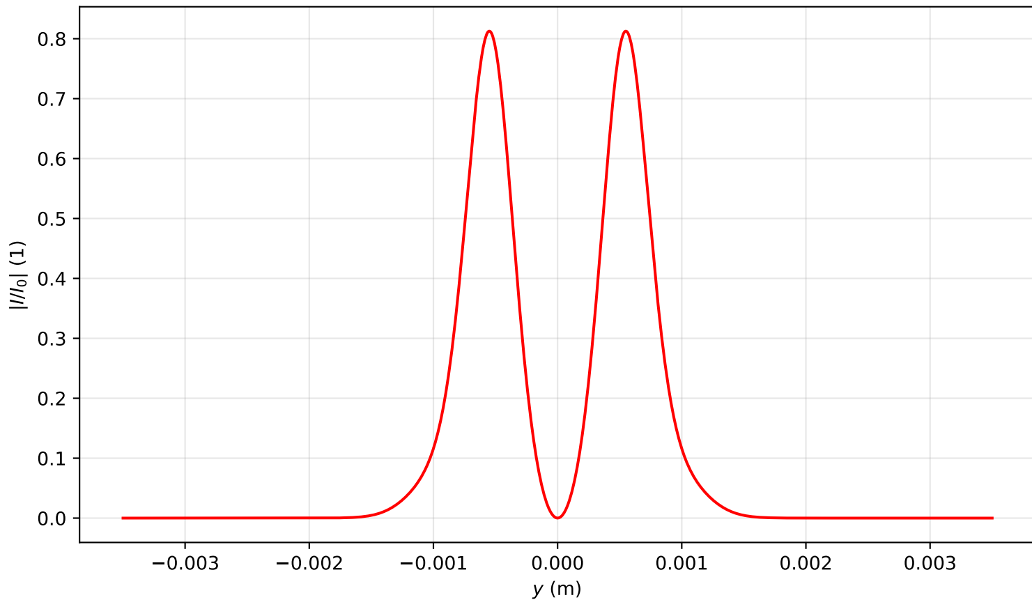
Intensity profile I(x=0, y, z=0.716)/I_0 , P_{in}=3.0P_{cr} , artificial time
